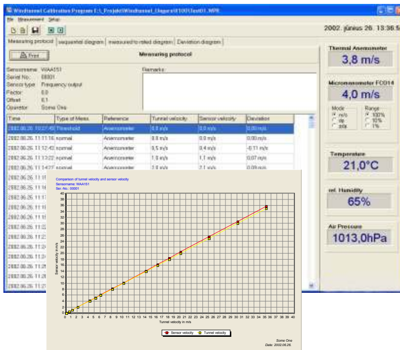
Example of numerical and graphical schemes of an anemometer characteristic
